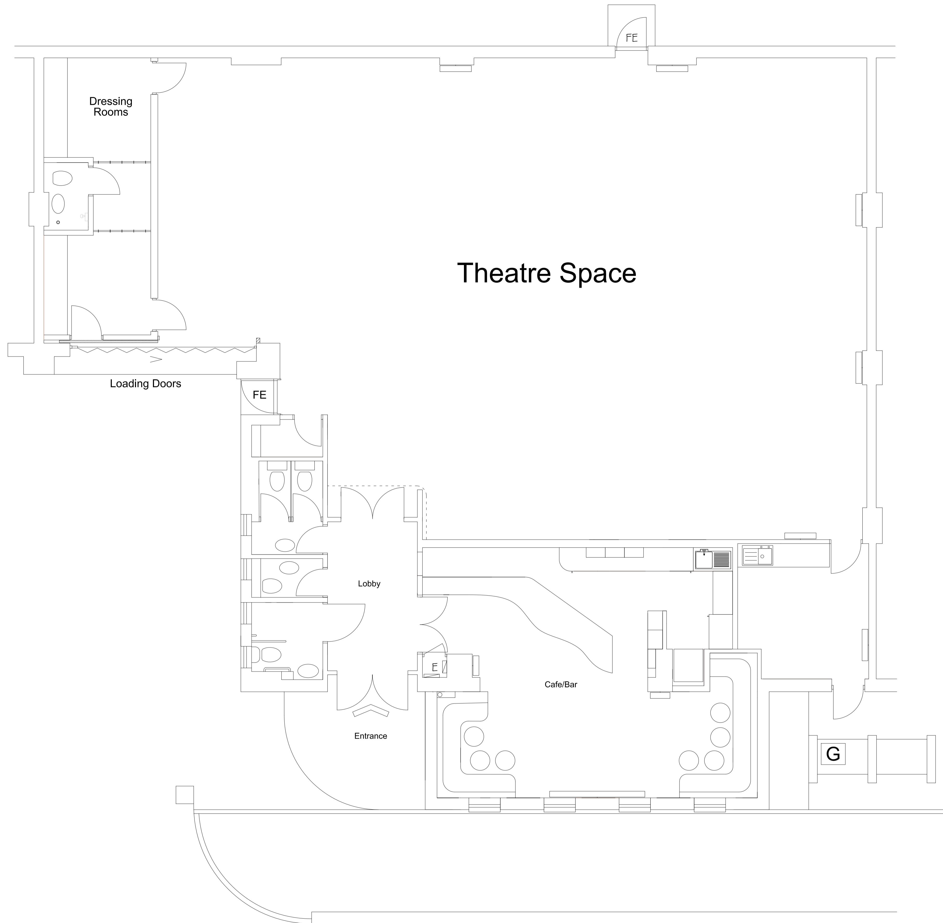
1 Floor Plan 1:50@ A1
